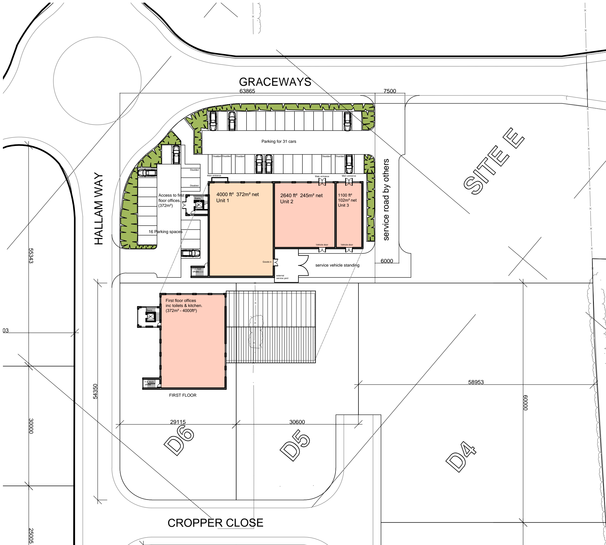
Proposed Block Plan @ 1:500 at A3
